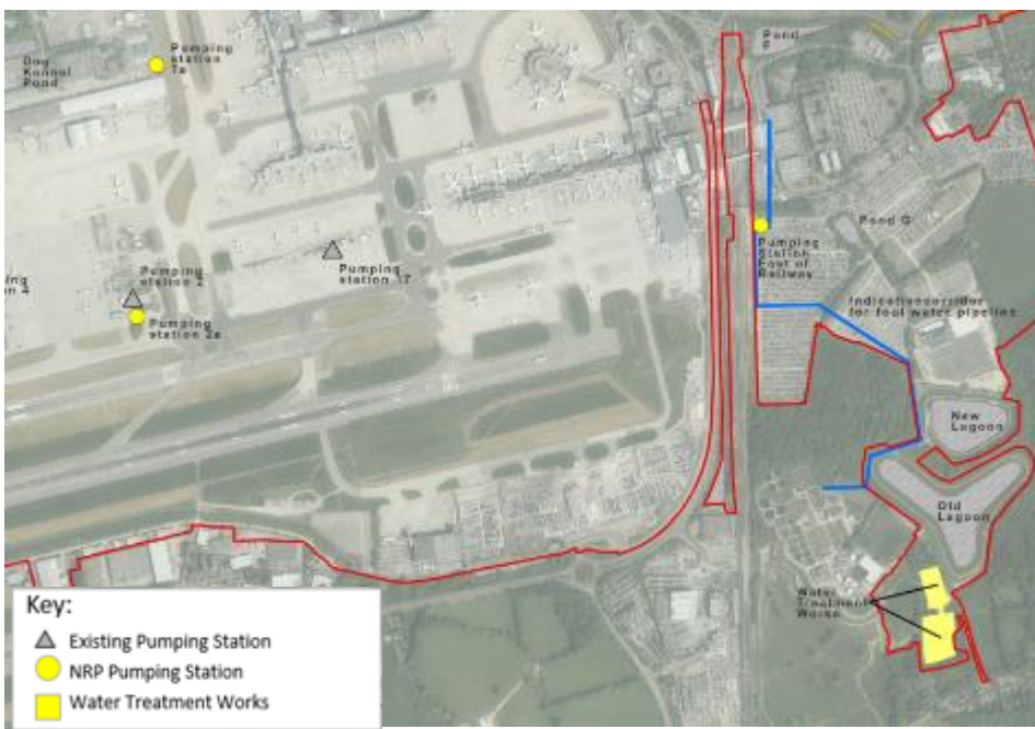
Figure 5757: Locations of proposed new pumping stations
