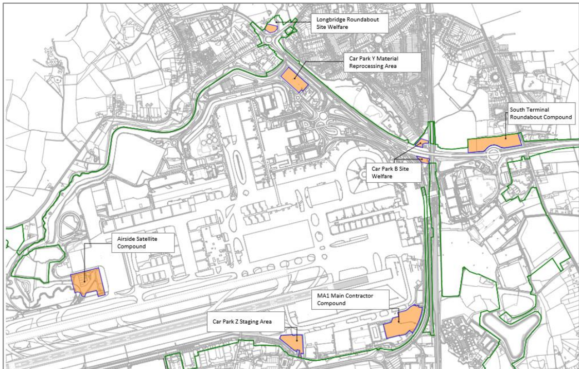
Figure 55: Anticipated locations of temporary construction compounds
