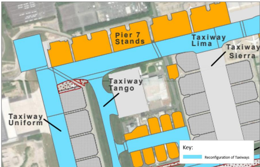
Figure 2020: Overview location of Taxiway Lima extension
