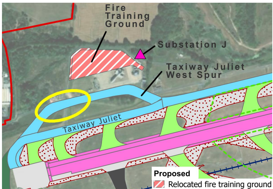
Figure 3333: Relocation of Fire Training Facility
