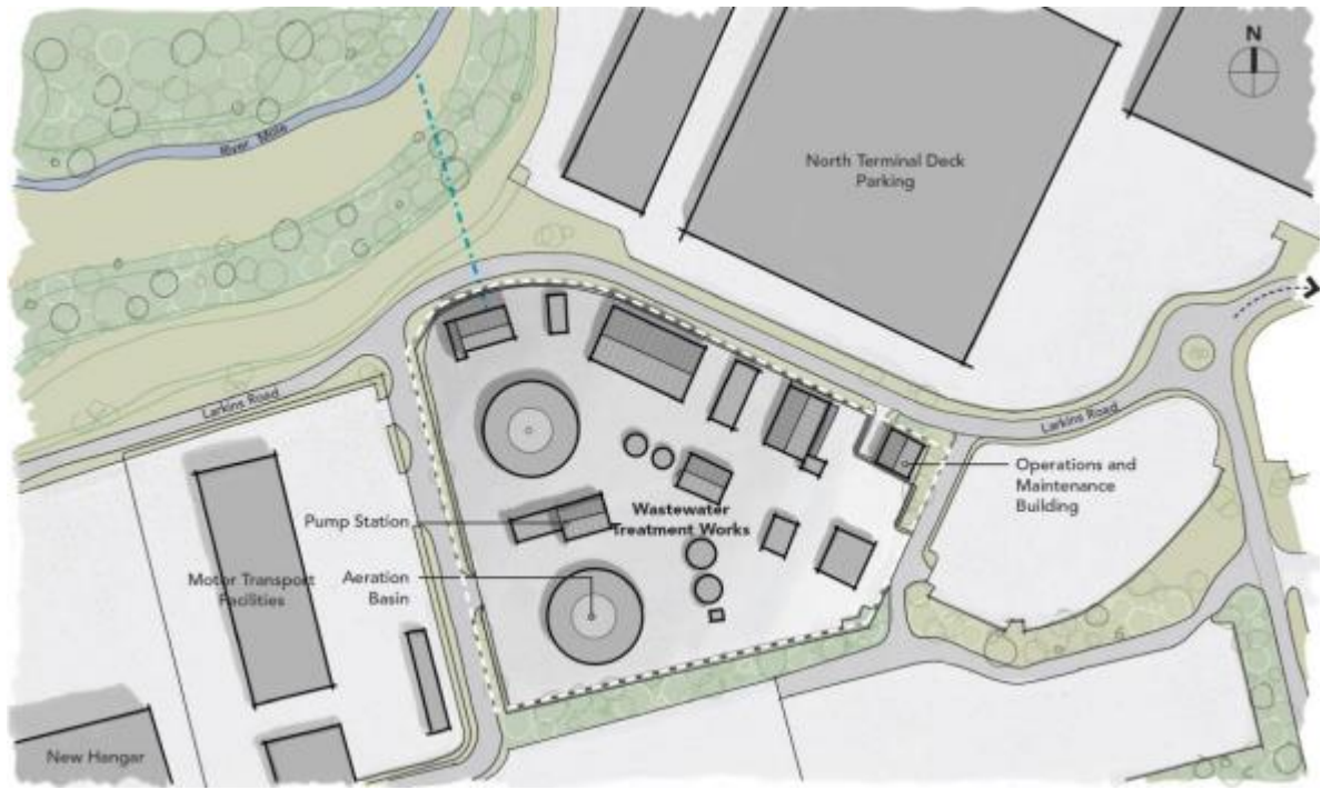
Figure 60: Indicative layout of the On-airport WWTW
