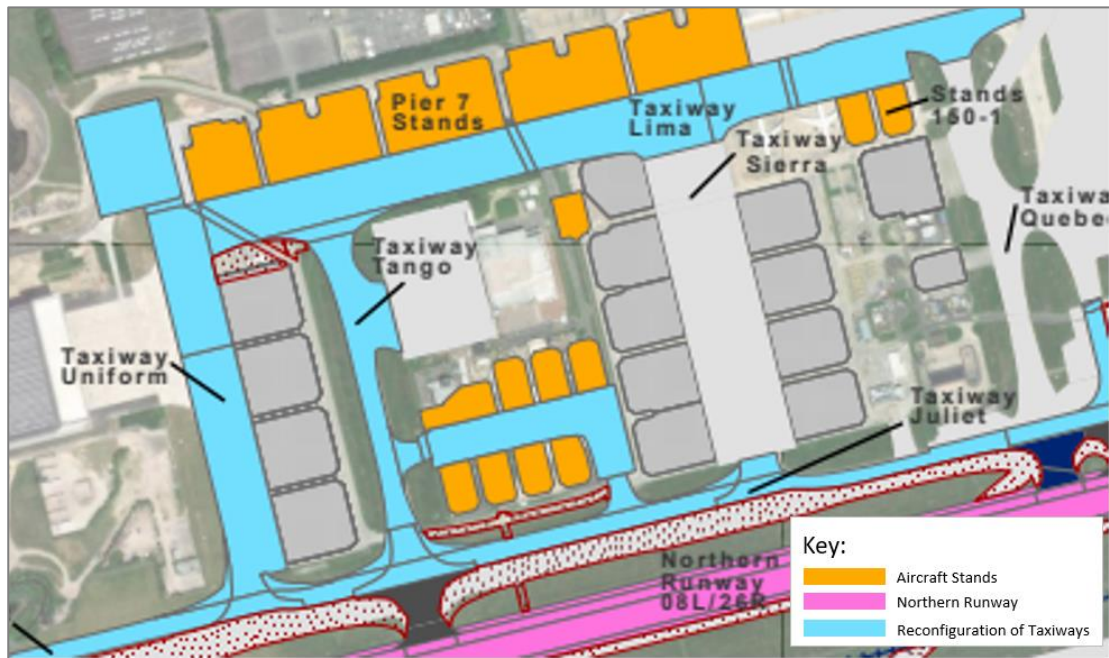
Figure 23.23: Aircraft stands
